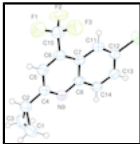
Fig. 1. The molecular structure of the title compound. Displacement ellipsoids are drawn at the 50% probability level. Hydrogen atoms are shown as spheres of arbitrary radius.
